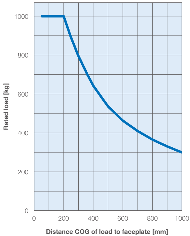
Maximum load of L-type positioner WL-500
