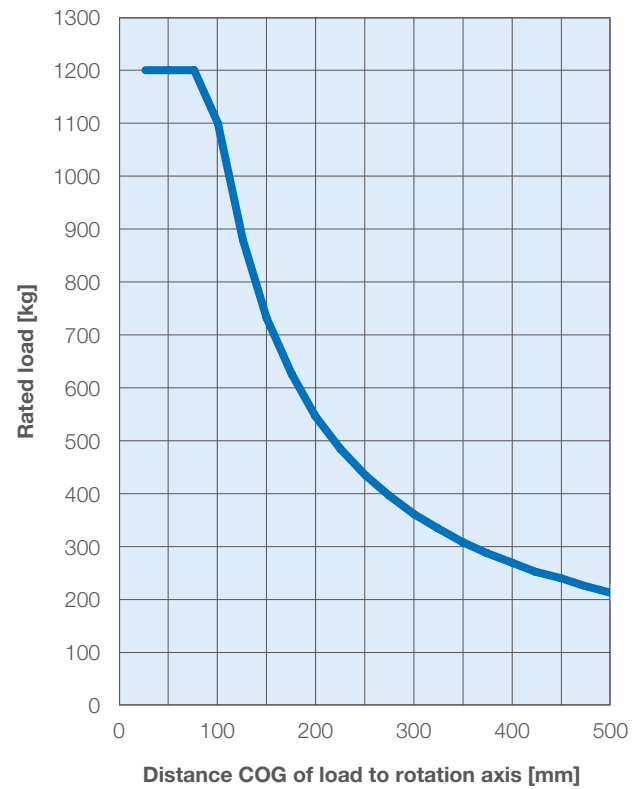
Maximum excentricity of load at rotation axis WL-500
