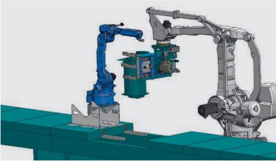
Highest flexibility for welding a wide range of different subassemblies with the ES280D II handling robot and MH24 welding robot Sensor technology: MOTOSense SeamFinder and tactile sensor
