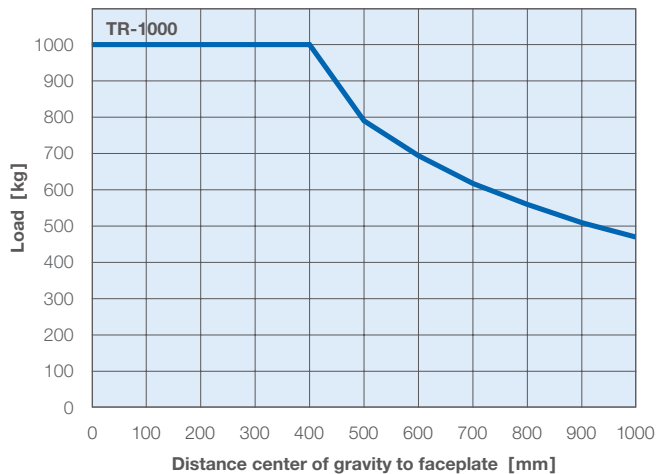
Load position – tilt-axis
