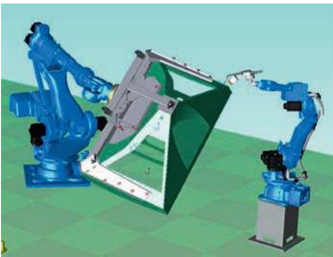
MAG welding on bulk material containers MH400 with MH50-30 Sensor technology: vision system, MOTOSense SeamFinder and tactile sensor
