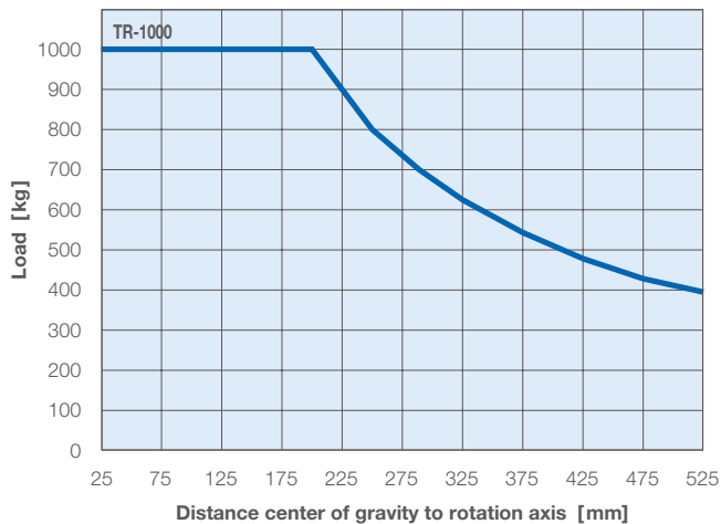
Load position – rotation-axis
